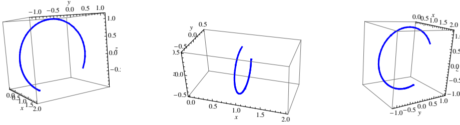
Figure 2: From left to right, the TN , TB and TNB Smarandache curves of \alpha .
