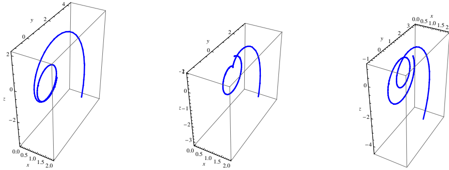
Figure 4: The TN , TB and TNB Smarandache curves of \delta .
