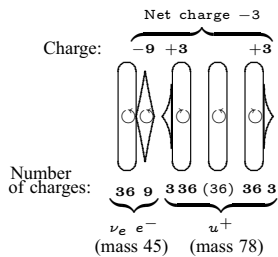
Fig. 6: Scheme of the d -quark. The symbol \diamond is used for the triplet ( e ), the symbols \{ and \} denote the tripoles ( Y -particles), and the symbols \square denote the hexaplets ( \nu_e ).
