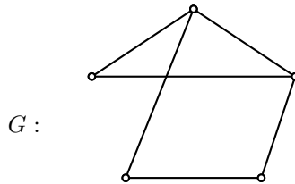
Fig.5.1 A graph G with \gamma(G^{+-+}) = \lceil n/2 \rceil .
