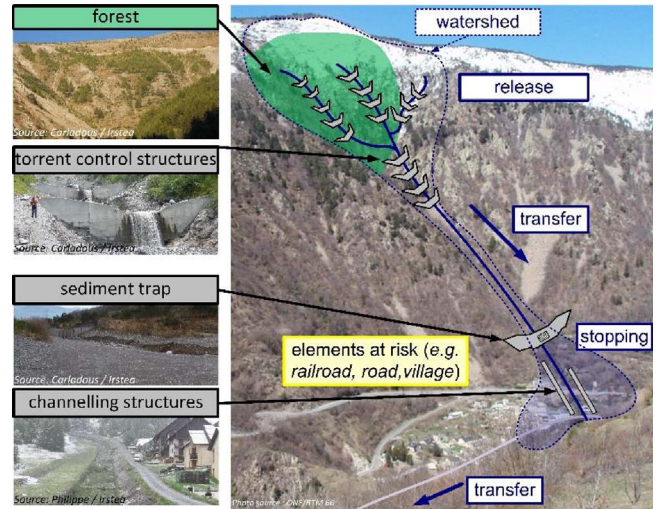
Fig. 2. Distribution of structural protection measures and their functions to mitigate torrential floods in a mountain watershed.
